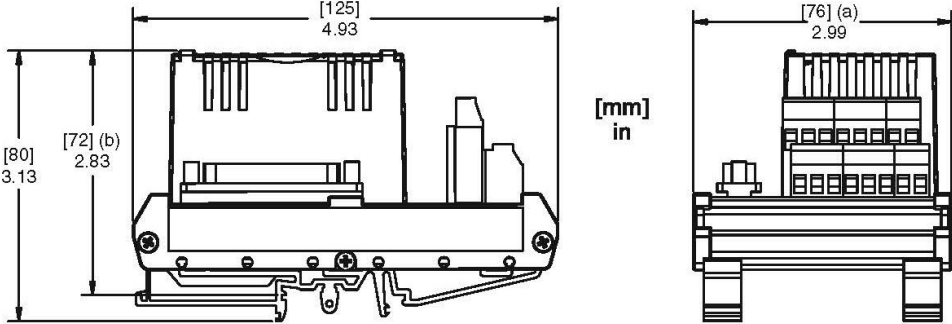
Compression Termination Assembly
