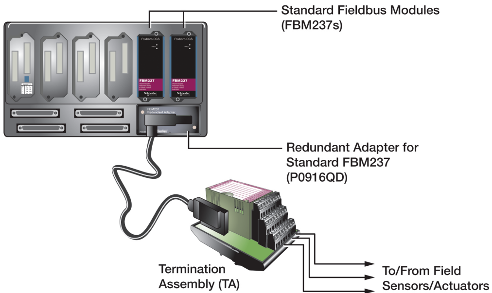
Figure 1 - Redundant I/O Configuration
